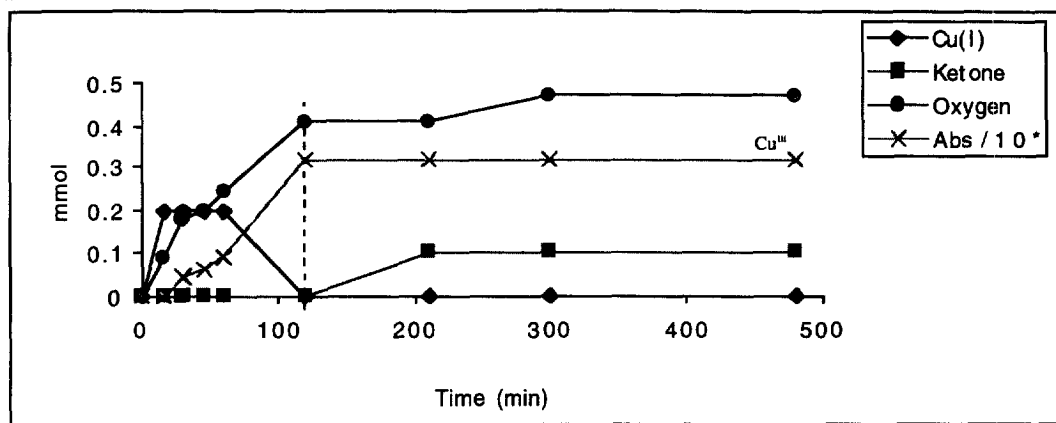
Chart 1: Kinetics of the parameters of the reaction using the \text{Cu}^{\text{II}}/\text{H}_2\text{O}_2 system.
