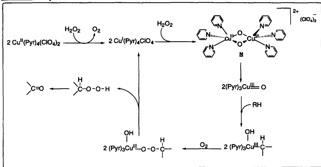
Scheme 1: Proposed mechanism
