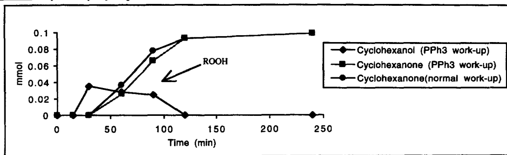
Chart 2: Cyclohexyl hydroperoxide is an intermediate.
