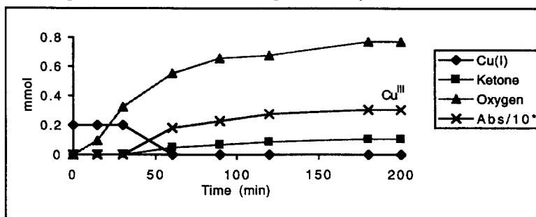
Chart 6: Kinetics of the parameters of the reaction using Cu I /H 2 O 2 system.
