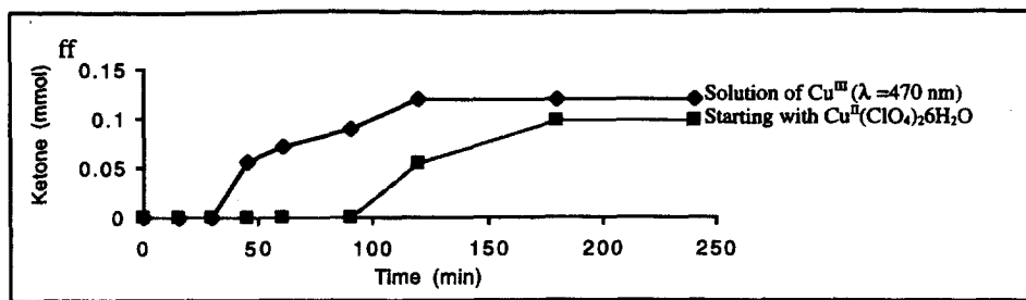
Chart 3: Kinetics of Ketone formation starting with the solution containing the active species.
